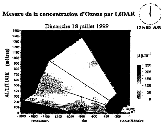
Fig. 5: Lidar location and typical mapping of 2D measurements.
