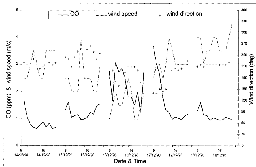
Figure 4: Time series of CO, with above-roof wind and direction
