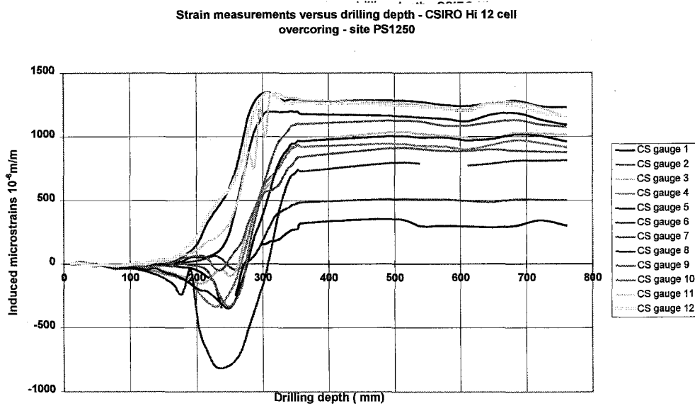
Fig. 2: (below) example of strains recorded during overcoring, on CSIRO Hi 12 cell., Final values are directly related to the insitu stress field. Compressive stresses found are (Bigarre, 1996) : (\sigma_1, \sigma_2, \sigma_3) = (-27, -19.5, -17.5) MPa.
