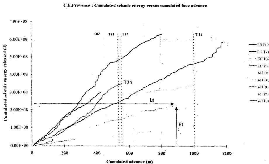
Figure 10 : plot of cumulative seismic energy release versus cumulated face advance concerning 9 panels from 4 different districts sparsed in the mine layout. Levels, trends and changes of seismic regime are routinely and comparatively examined in order to classify current working faces.
