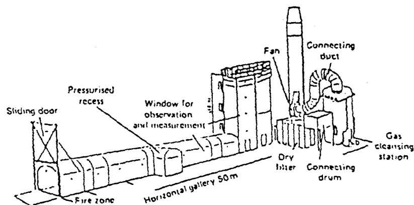
Figure 1 : view of the INERIS fire test gallery
