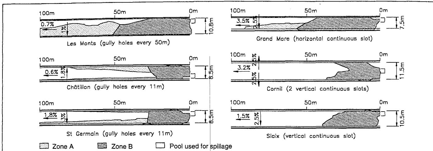
Fig. 3: Wet zones A and B for a sudden spillage of 10 m³
