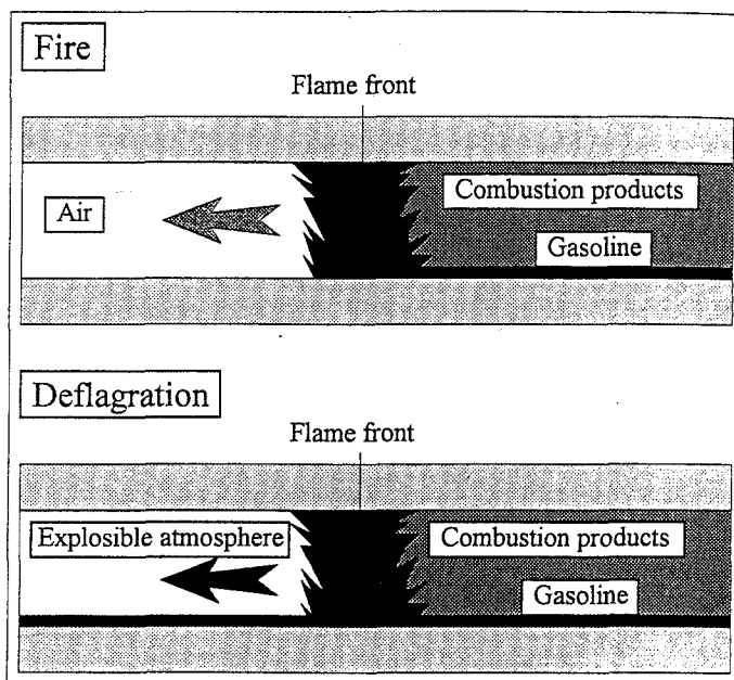
Fig. 8: Combustion process in the collector
