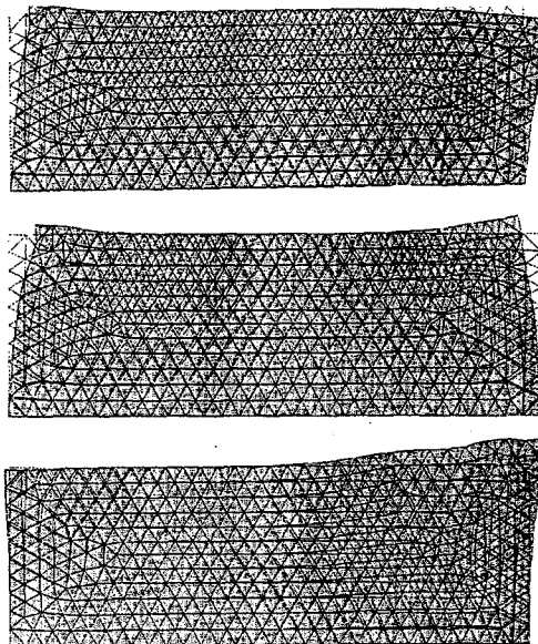
Figure 4. The first three mode shapes of the model determined by a finite element modal analysis.
