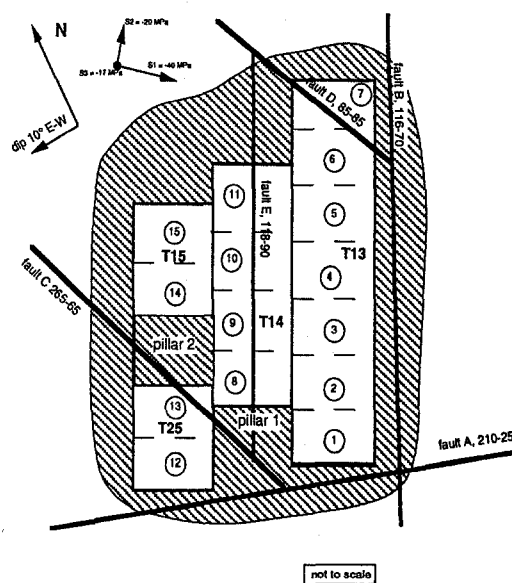
fig. 6 - modeling of the Estaque sud district faults are indicated with dip direction and dip
