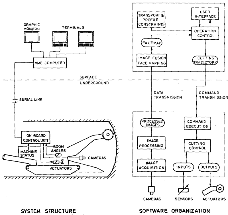
Figure 7. Control system structure
