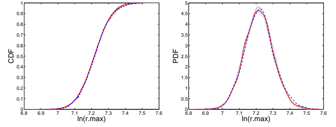
Figure 7: Response CDF (left panel) and kernel density estimated PDF (right panel) for: 1000 standard Monte Carlo simulation (dotted blue line), meta-model simulation through PCE (solid red line), replicated meta-model simulation (dark grey lines).
