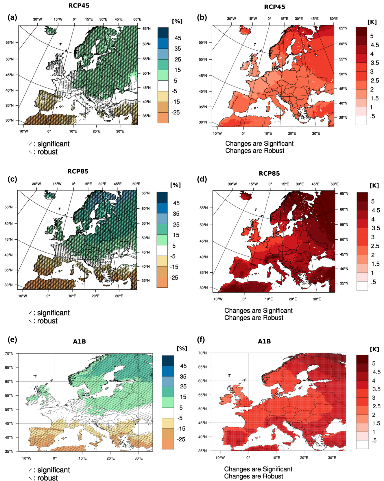
Fig. 1 Projected changes of total annual precipitation (%) (left) and annual mean temperature [K] (right) for 2071–2100 compared to 1971–2000, for A1B (e, f), RCP8.5 (c, d) and RCP4.5 (a, b) scenarios.
