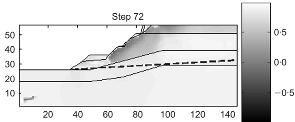
Fig. 18. Isovalues of the second-order work in the Trevoux slope at step 72 of the rising water table (dashed line)
