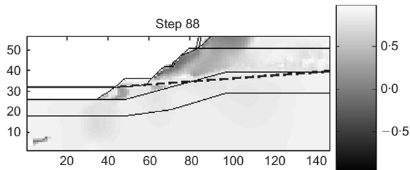
Fig. 19. Isovalues of the second-order work in the Trevoux slope at step 88 of the rising water table (dashed line)
