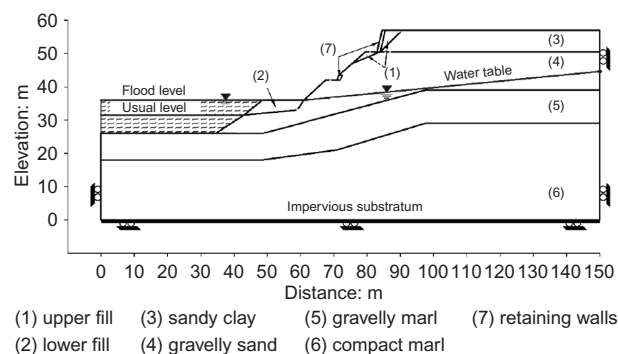
Fig. 2. Typical cross-section of the Trevoux landslide
