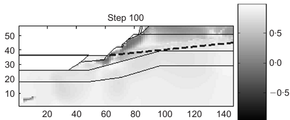
Fig. 20. Isovalues of the second-order work in the Trevoux slope at step 100 of the rising water table (dashed line)
