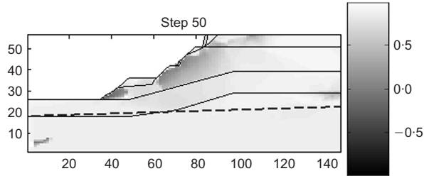
Fig. 17. Isovalues of the second-order work in the Trevoux slope at step 50 of the rising water table (dashed line)
