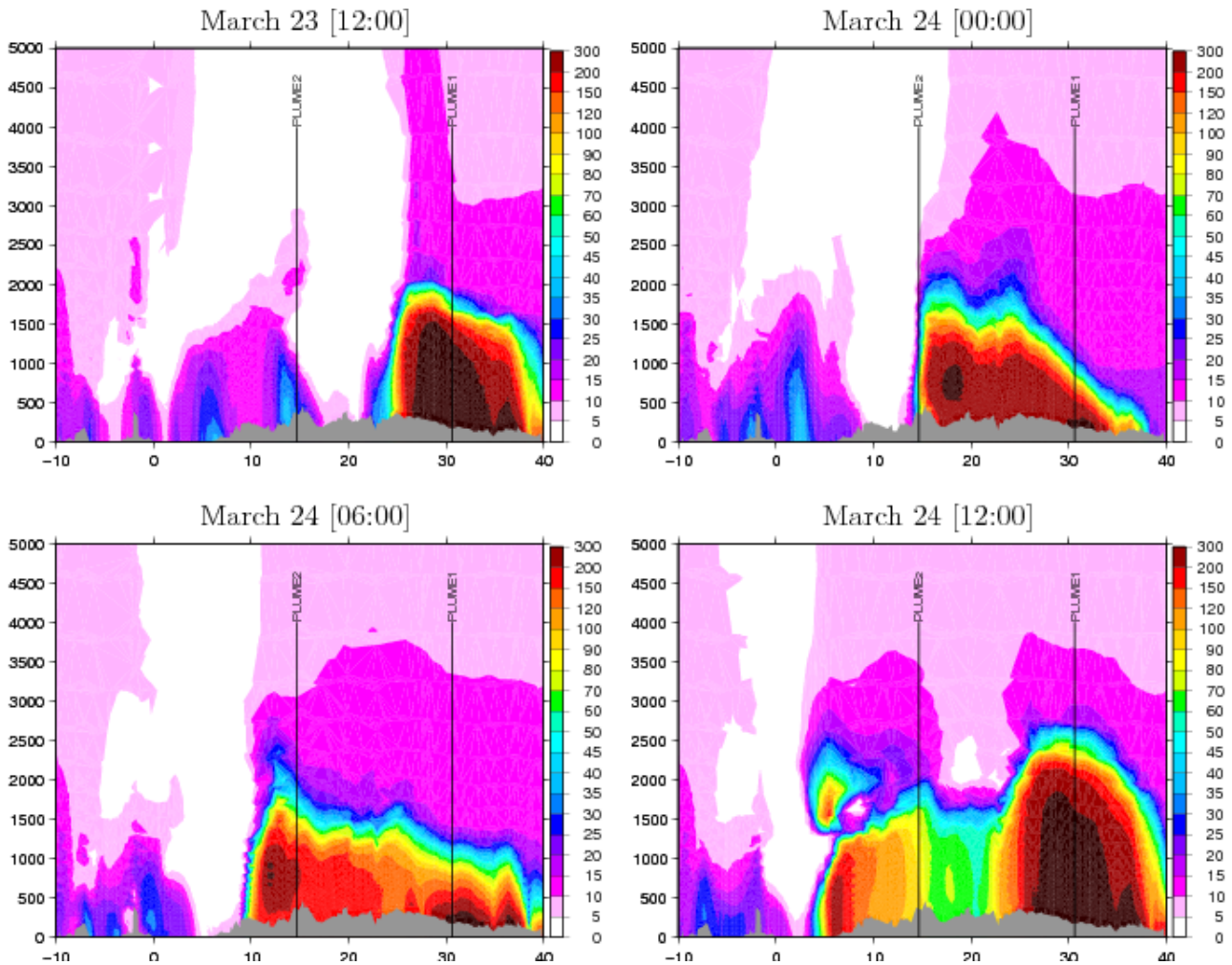
Figure 11. Vertical cross-section (Longitude-Height diagrams) of PM10 concentrations ( \mu\text{g}\cdot\text{m}^{-3} ) along the plume (straight line passing through PLUME1 and PLUME2). The two arbitrary points named PLUME1 ( 30.6^{\circ}\text{E}-48.7^{\circ}\text{N} ) and PLUME2 ( 14.6^{\circ}\text{E}-51.0^{\circ}\text{N} ) represent respectively the emission area and a point located over the plume trajectory. Color scale stops at 300 \mu\text{g}\cdot\text{m}^{-3} , even if some very important values are calculated.
