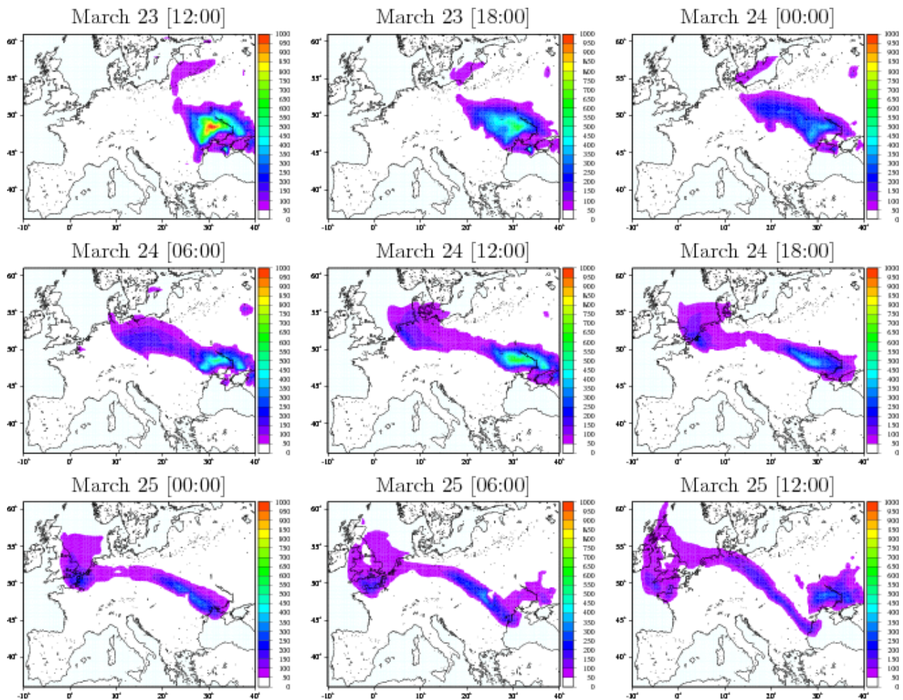
Figure 10. Surface PM 10 concentrations ( \mu\text{g}\cdot\text{m}^{-3} ) simulated by CHIMERE from March 23 [12:00] to 25 [12:00], 2007 (see Table 1 for the names of the stations).
