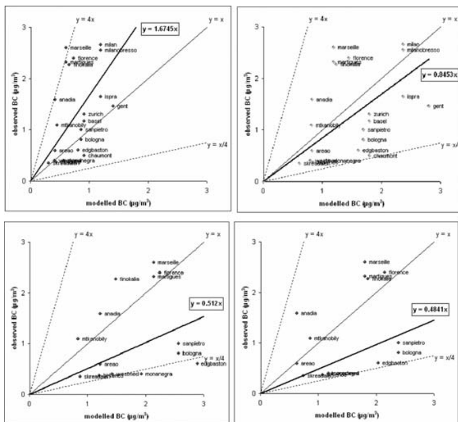
Fig. 10. Scatter plot diagrams of modelled vs. observed BC concentrations (in \mu\text{g m}^{-3} ) for summer 2022 in the (a) S1, (b) S2, (c) S3 and (d) S4 simulations.
