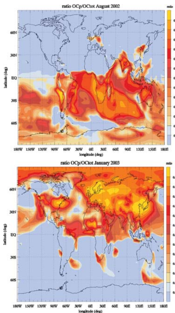
Fig. 13. OCp/OCtot ratios in August 2002 and January 2003.
