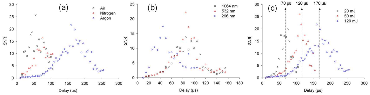
Figure 10. LIBS signal temporal evolution for (a) three different background gas, E_{\text{laser}} = 120 \text{ mJ} , \lambda = 1064 \text{ nm} (b) three different laser wavelengths, argon as background gas and E_{\text{laser}} = 30 \text{ mJ} (c) three different laser energies, argon as background gas and \lambda = 1064 \text{ nm} . These plots were obtained when analyzing polydisperse flows of aluminium particles with sizes ranging from 10 to 200 nm and a median diameter of 30 nm. Temporal resolution was obtained using 500 ns gate width and by accumulating spectra over 800 laser shots.
