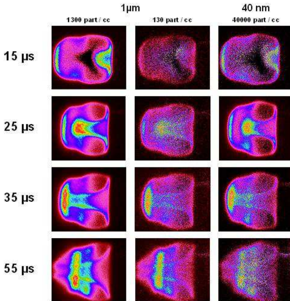
Figure 3. Spatio-temporal evolution of sodium chloride vaporized matter visualized using spectral images acquired over 200 and 100 laser sparks when vaporizing 40 nm and 1 \mu m sized particles respectively. Time delays and particle numbers are indicated on the figure. Laser energy was set to 120 mJ.
