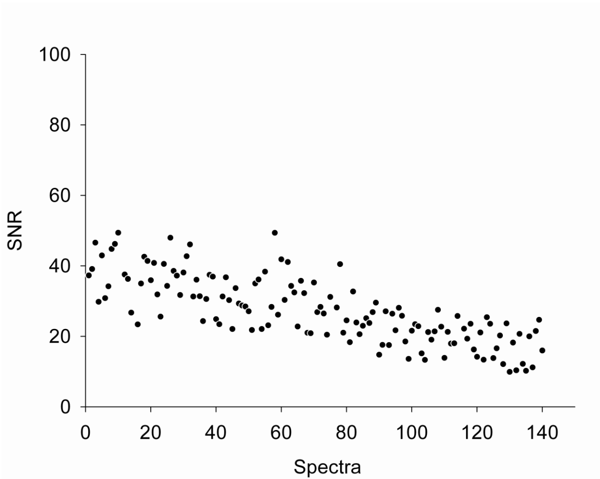
Figure 8. LIBS signal variability in the course of spectra recording. The drop in particle concentration causes the LIBS intensity to decrease. This plot was obtained when irradiating monodisperse flows of sodium chloride particles with sizes of 400 nm and particle number varying from 3500 to 1000 particles per cubic centimeters. Time delay of 40 \mu s, gate width of 100 \mu s and 10,000 accumulations were used as LIBS experimental parameters. The laser energy was set to 120 mJ.
