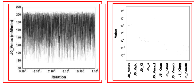
Fig. 2. Trajectory of 3 Markov chains for parameter J0\_Vmax at convergence over the last half-million runs (left); On the right: percentile plot (5 th , 25 th , 50 th , 75 th and 95 th percentiles) of the posterior sample obtained for each parameter, overlaid with their "true" value (crosses).
