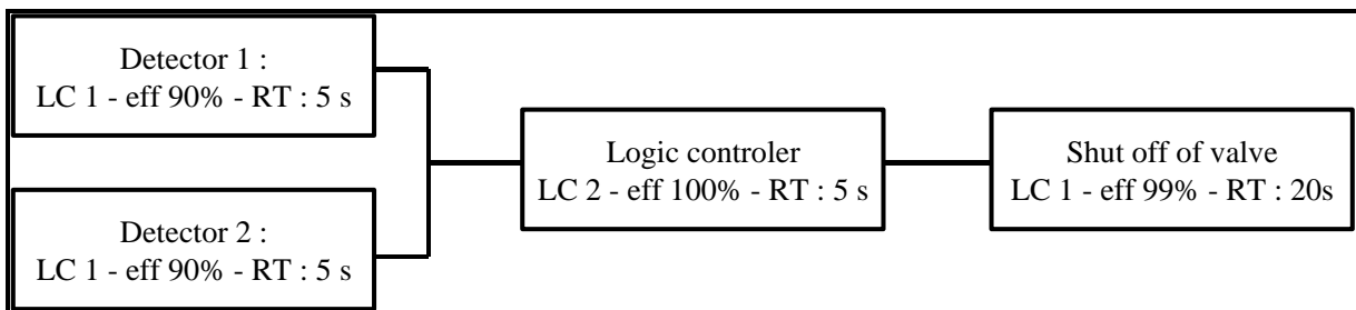
Figure 12: Architecture of safety function (LC1 - eff. 90% - RT: 30s)
