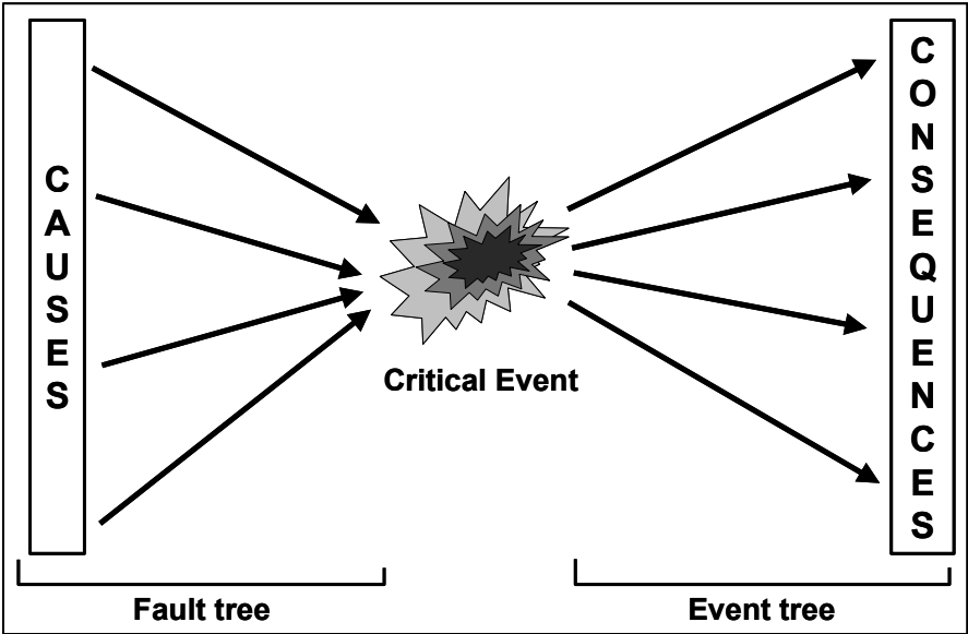
Figure 1: General scheme of the bow-tie
