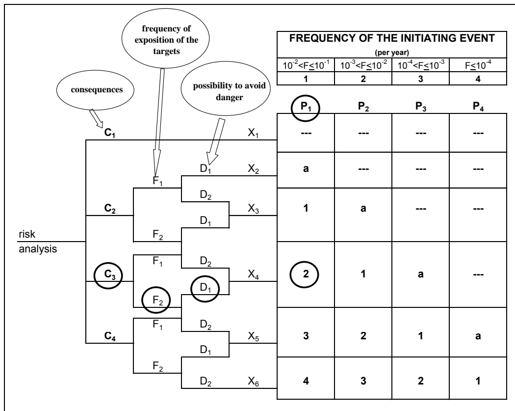
Figure 14: Risk graph for the scenario – cause “operator error” – residual scenario
