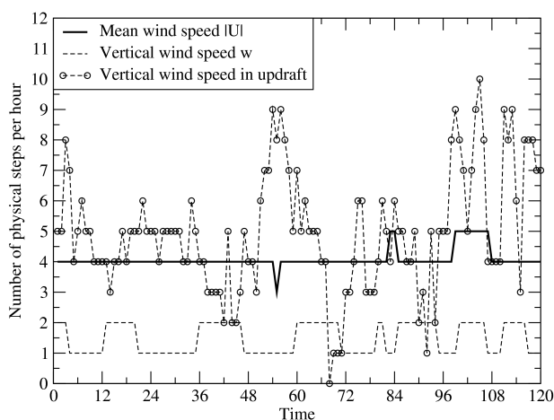
Fig. 3. Calculation of the number of integration steps per hour to respect the Courant–Friedrich–Levy (CFL) number over a complete 120 h simulation. The CFL is estimated using three parameters: the mean wind speed |U| , the vertical wind speed in the environment w , and the vertical velocity in the updraft in case of active deep convection.
