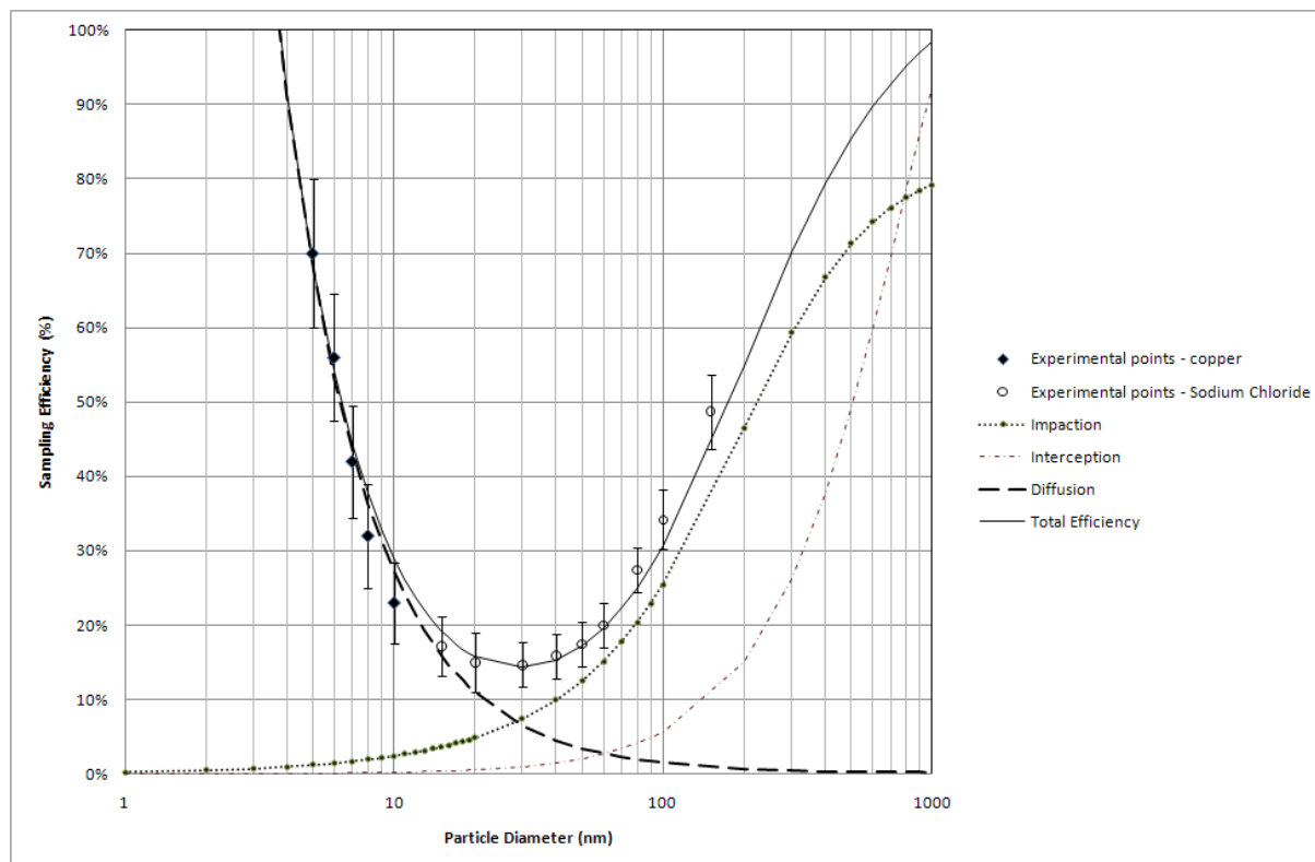
Figure 7: Comparison of experimental and theoretical approaches to assessing collection efficiency of the Quantifoil 1.2/1.3 TEM grid.
