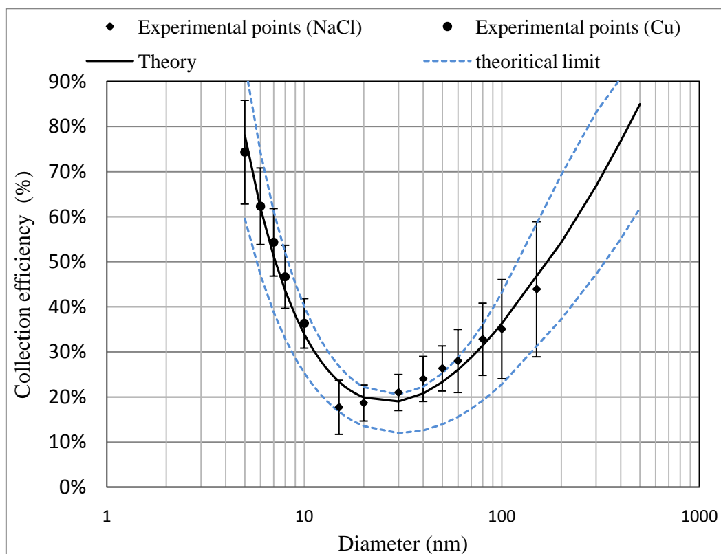
Figure 6: Particle collection efficiency by size for the Holey TEM grid. The theoretical collection efficiency has been calculated using the parameters related to the operation conditions and characteristics of the TEM grid (cf. Table 1).
