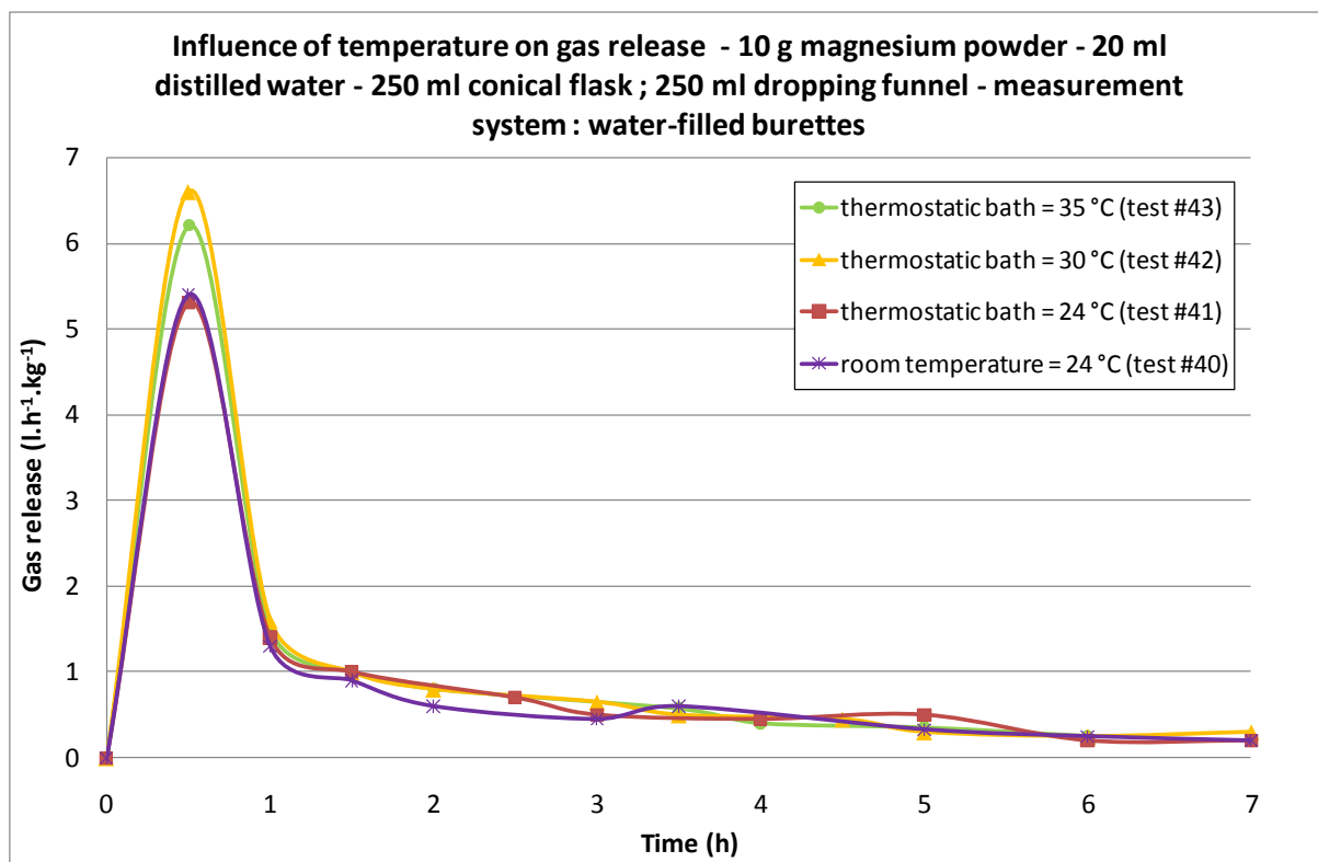
Figure 2: Influence of temperature on gas release – magnesium powder
