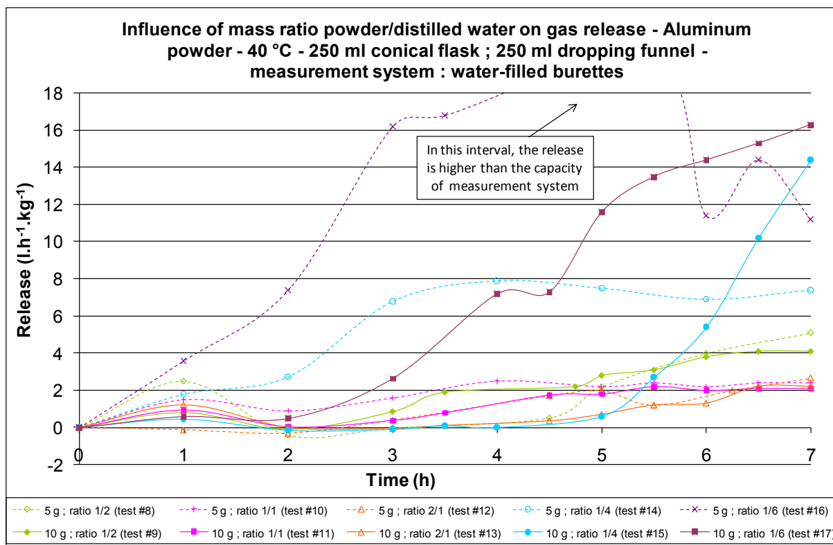
Figure 4: Influence of mass ratio powder/distilled water, aluminum powder
