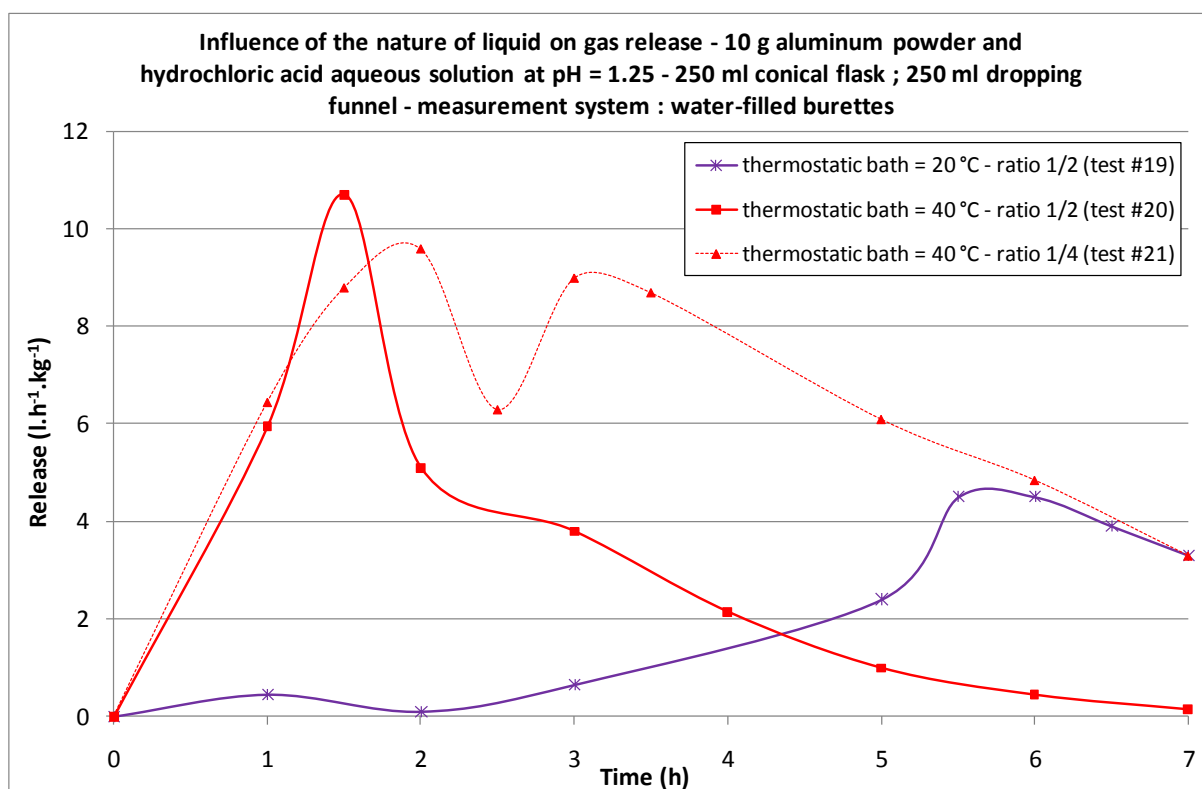
Figure 8: Influence of the nature of the liquid on gas release, aluminum and hydrochloric acid at pH = 1.25
