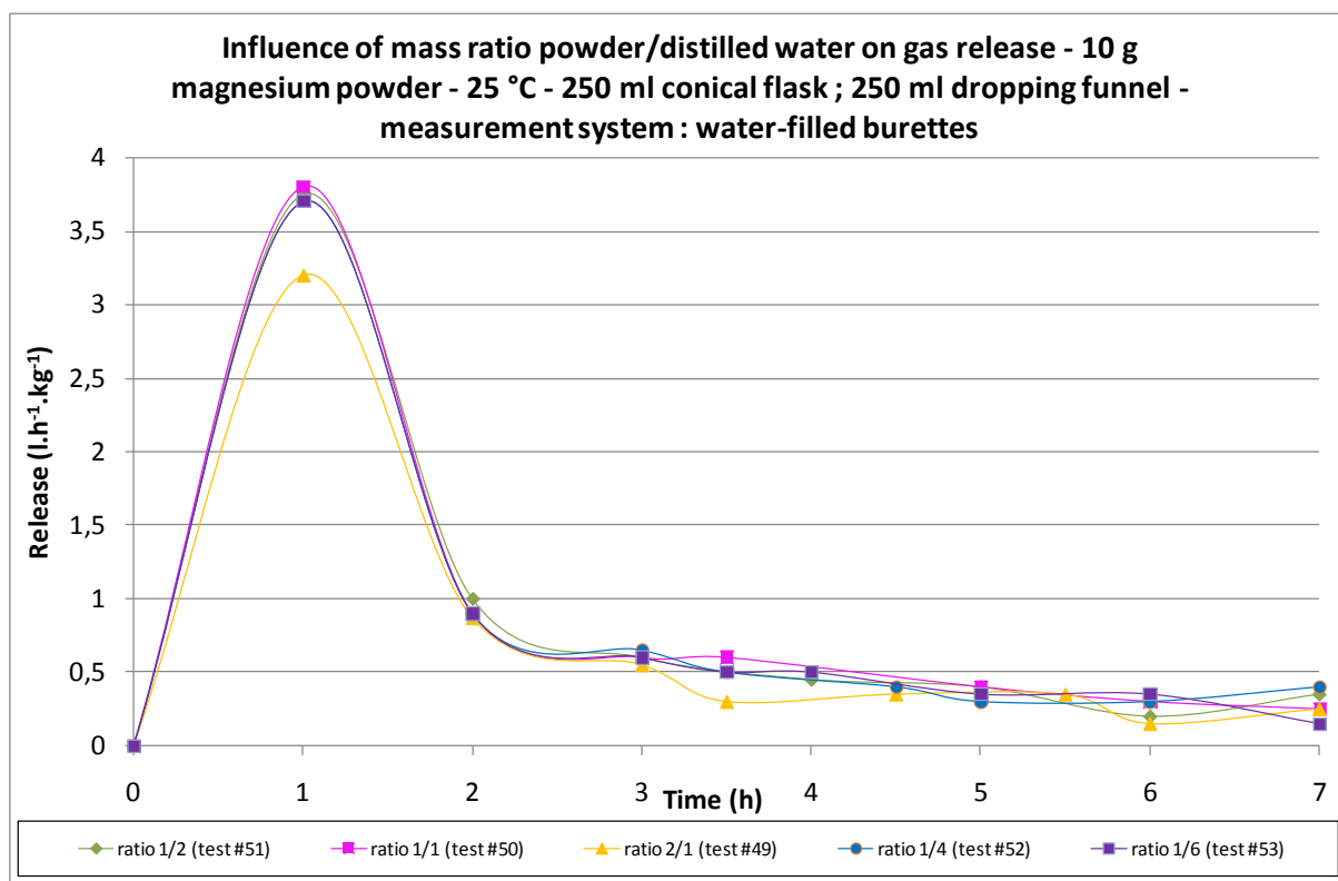
Figure 5: Influence of mass ratio powder/distilled water, magnesium powder
