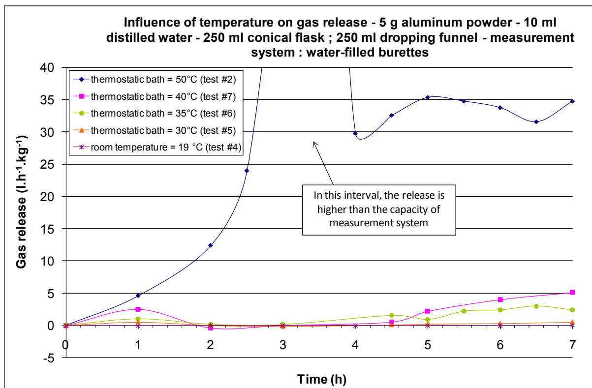
Figure 1: Influence of temperature on gas release – aluminum powder
