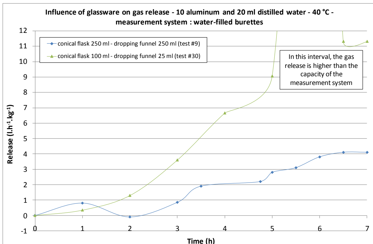
Figure 12: Influence of glassware on gas release, 10 g aluminum, and mass ratio 1/2
