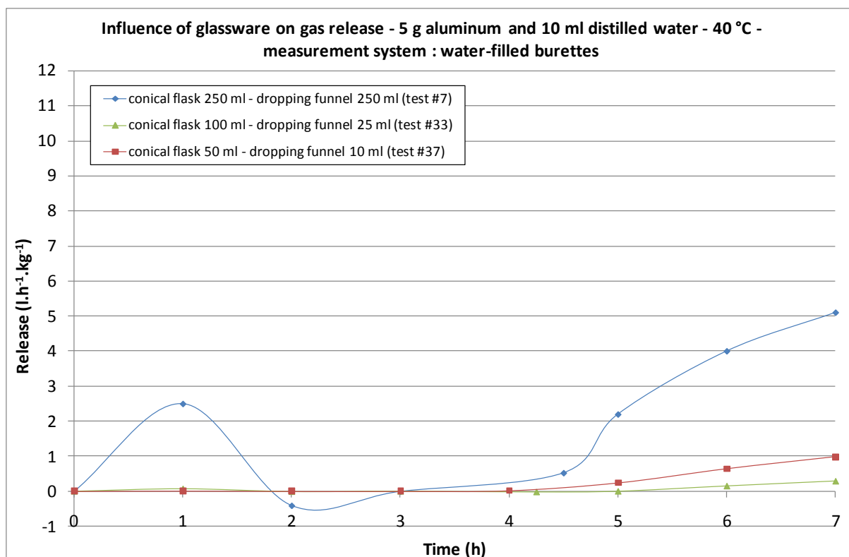
Figure 11: Influence of glassware on gas release, 5 g aluminum, and mass ratio 1/2
