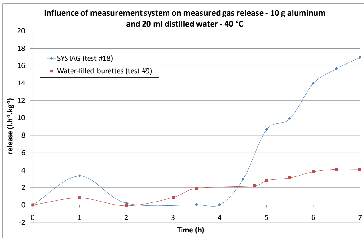
Figure 15 : Influence of measurement system on measured gas release, 10 g aluminum and mass ratio 1/2
