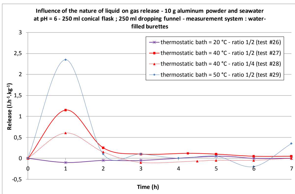
Figure 6: Influence of the nature of the liquid on gas release, aluminum and seawater
