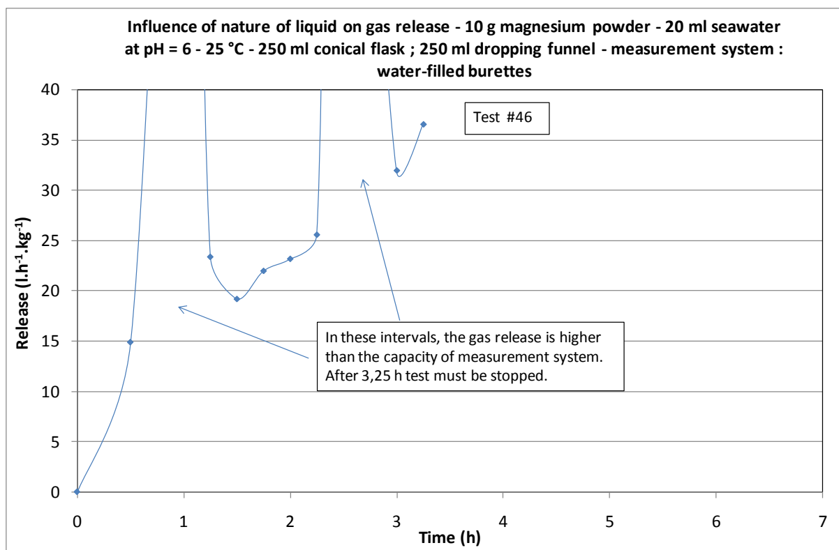
Figure 7: Influence of the nature of the liquid on gas release, magnesium and seawater
