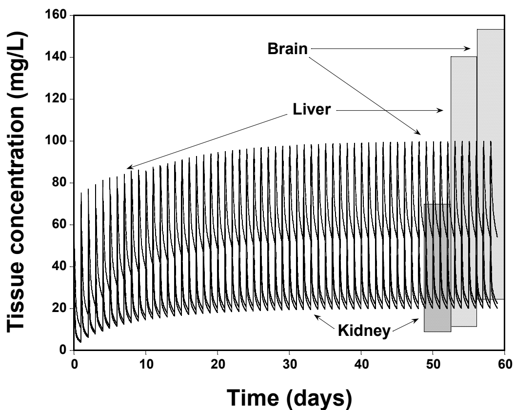
Fig. 7: Predictions of long-term ciclosporin A pharmacokinetics in humans.
