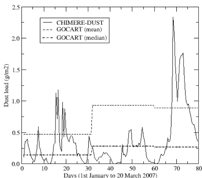
Fig. 3. Comparisons of monthly GOCART climatology and hourly CHIMERE-DUST dust loads. Surface concentrations for a grid cell over the Mediterranean sea and used as boundary conditions for actual European domains forecast modeling.
