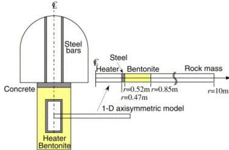
Fig. 4. Geometry of the simplified axisymmetric model.
