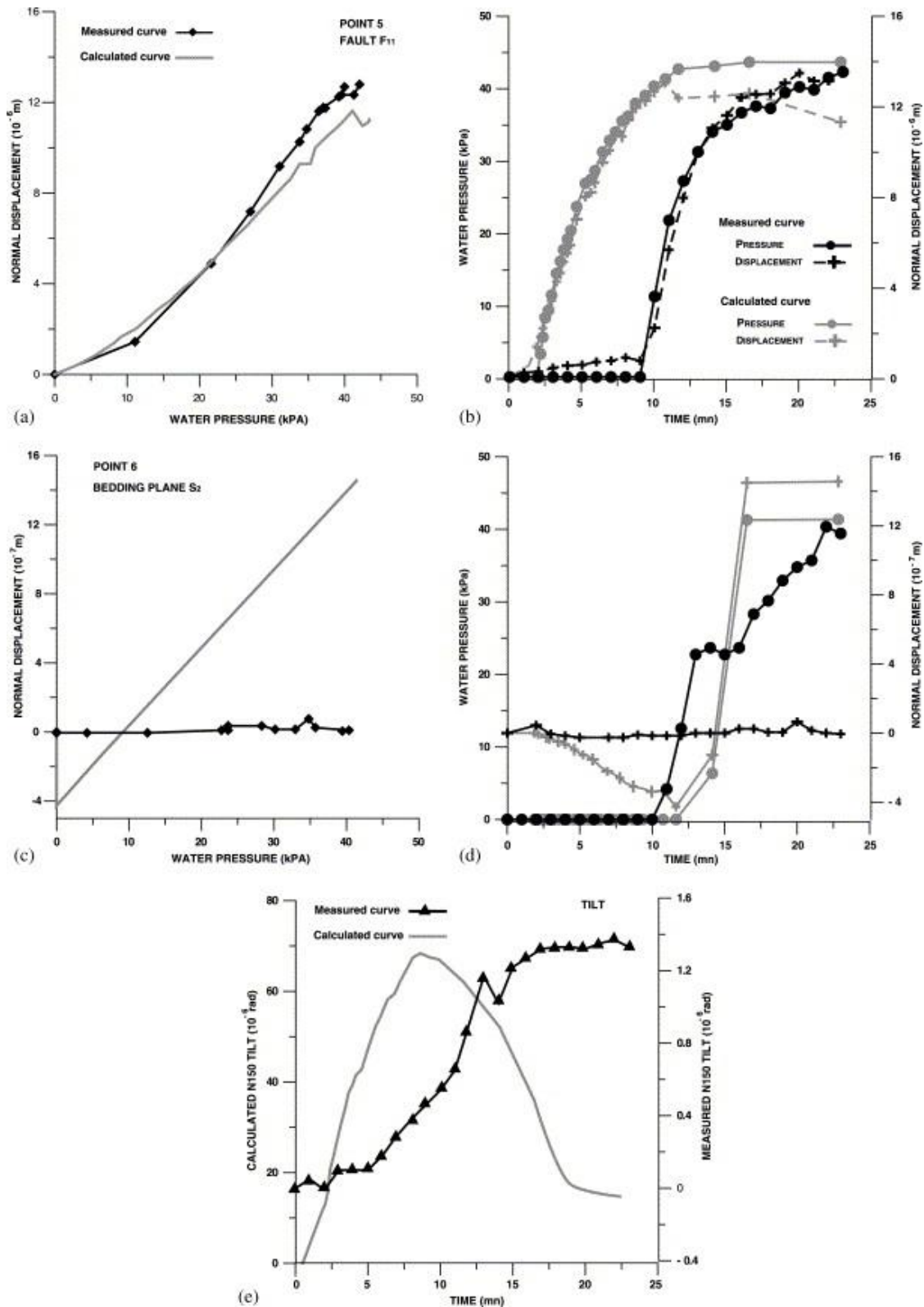
Fig. 7. Reference case of hydromechanical modelling. (a) Normal displacement versus water pressure at point 5 of fault F 11 . (b) Normal displacement and water pressure versus time at point 5 of fault F 11 . (c) Normal displacement versus water pressure at point 6 of bedding plane S 2 . (d) Normal displacement and water pressure versus time at point 6 of bedding plane S 2 . (e) N150 tilt versus time (left vertical axis corresponds to calculated N150 tilt—right vertical axis corresponds to measured N150 tilt).
