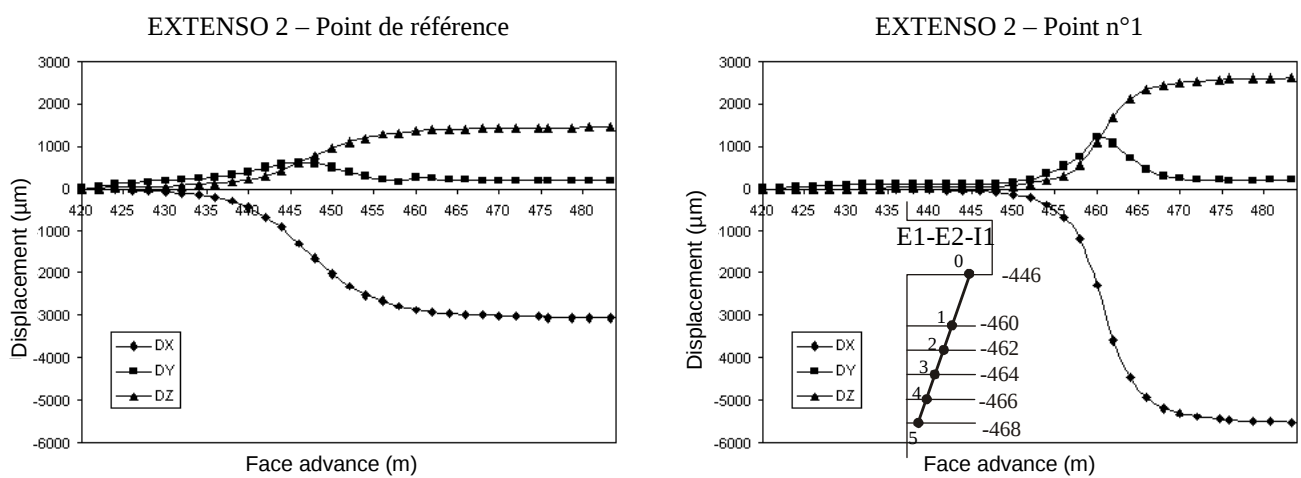
Figure 3 : Comparison between displacements of the n°1 measurement and reference points of extensometer 2
